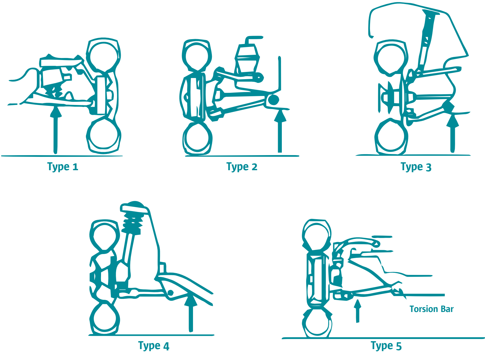
Figure 3. Suspension Types
